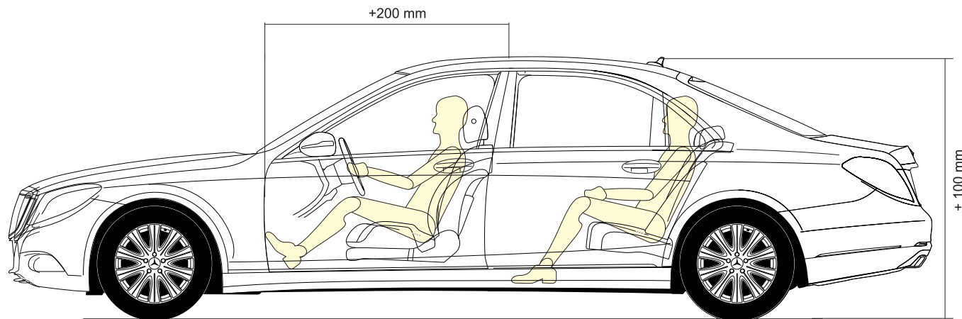
MERCEDES S CLASS MAYBACH STRETCHED BY 20 CM (+20+0 (EWB)) AND ROOF RAISED BY 10 CM
