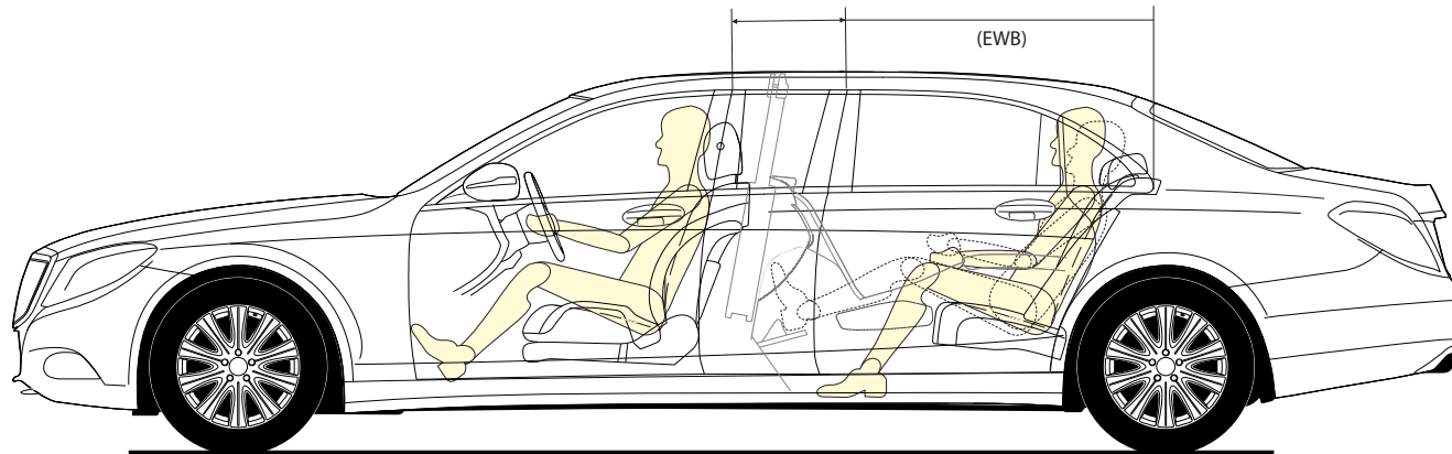
MERCEDES S CLASS MAYBACH STRETCHED BY 50 CM (+50+0 (EWB)) AND ROOF RAISED BY 10 CM
