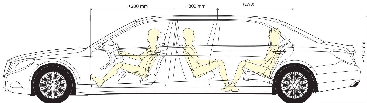
MERCEDES S CLASS MAYBACH STRETCHED BY 100 CM (+20+80+0 (EWB)) AND ROOF RAISED BY 10 CM
